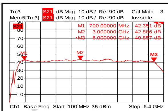
增益 (+85℃)
