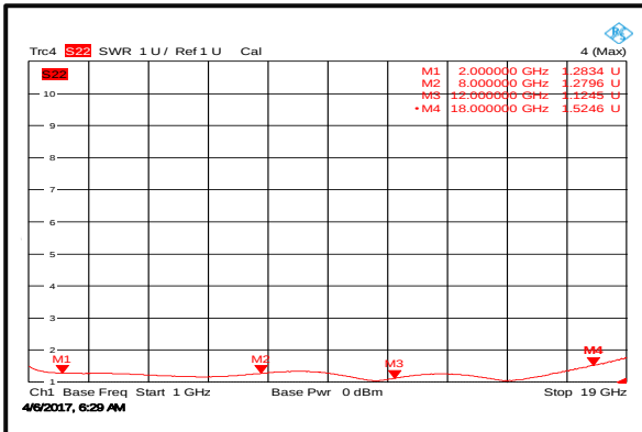
输出驻波比 (+25℃)
