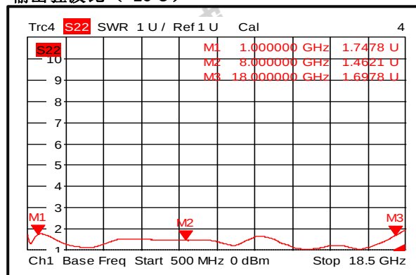
输出驻波比 (+25℃)
