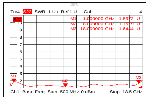
输出驻波比 (+85℃)
